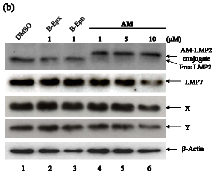
Figure 4.2 Selective modification of LMP2 in PC3 cell line. (a) Competition assay. PC3 cells were pre-treated with AM before the addition of biotin-tagged dihydroeponepmycin to visualize the catalytic subunits that were not targeted by AM. (b) Mobility shift assay. PC3 cells were treated with the indicated concentrations of AM, biotin-epoxomicin (B-Epx) and biotin-dihydroeponepmycin (B-Epn) for 1.5 hours. The mobility shift of the catalytic subunits were then analyzed by western blot using anti-LMP2, -LMP7, -X and -Y antibodies.
